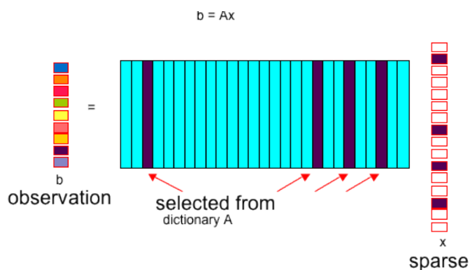
Figure 1: Sparse representation of a signal \mathbf{b}
